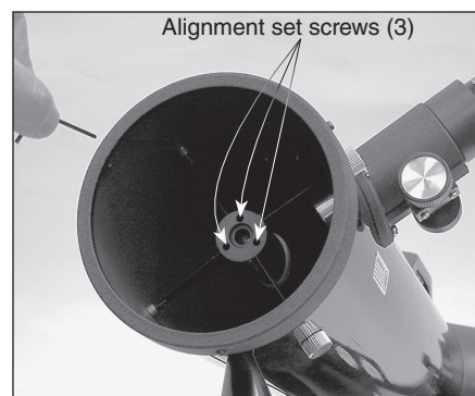
Figure 14. Adjust the tilt of the secondary mirror by loosening one of the three alignment set screws then tightening the other two.
