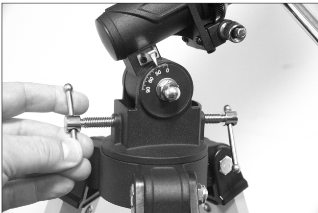
Figure 2. Attach the EQ head to the tripod by threaded the large thumb knob up from below until the EQ head is snug against the tripod.
