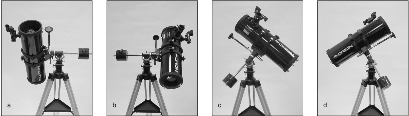
Figure 10. This illustration shows the telescope pointed in the four cardinal directions (a) north (b) south (c) east (d) west. Note that the tripod and mount have not been moved; only the telescope tube has been moved in the R.A. and Dec. axes.
