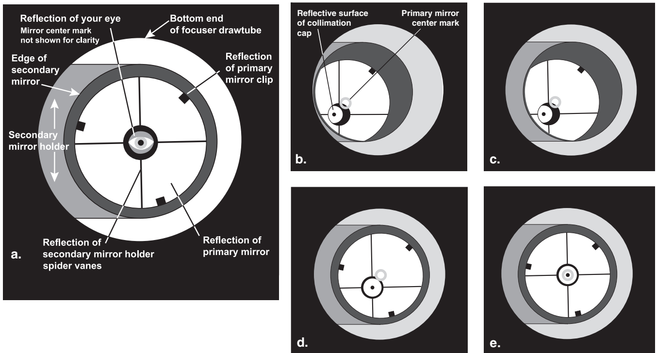
Figure 11. Collimating the optics. (a) When the mirrors are properly aligned, the view down the focuser drawtube should look like this. (b) With the collimation cap in place, if the optics are out of alignment, the view might look something like this. (c) Here, the secondary mirror is centered under the focuser, but it needs to be adjusted (tilted) so that the entire primary mirror is visible. (d) The secondary mirror is correctly aligned, but the primary mirror still needs adjustment. When the primary mirror is correctly aligned, the “dot” will be centered, as in (e) .
