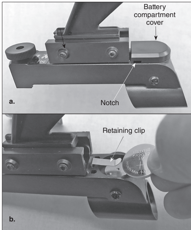
Figure 6. a) To install the CR2032 battery in the EZ Finder II, first turn it upside-down and remove the battery compartment cover. b) Install the battery with positive (+) side facing outward, as shown.
