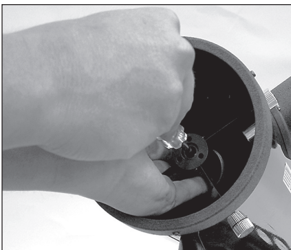
Figure 13. To center the secondary mirror under the focuser, hold the secondary mirror holder in place with your fingers while adjusting the center screw. Do not touch the mirror's surface.
