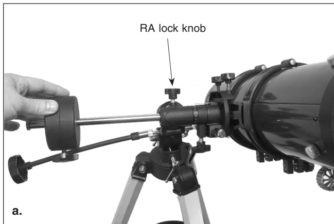
Figure 4. Proper usage of the equatorial mount requires the telescope tube to be balanced on both the R.A. and Dec. axes. (a) With the R.A. lock knob released, slide the counterweight along the counterweight shaft until it just counterbalances the tube. When you let go with both hands, the tube should not drift up or down. (b) With the Dec. lock knob released, loosen the tube ring lock clamps a few turns and slide the telescope forward or back in the tube rings. When the tube is balanced about the Dec. axis, it will not move when you let go.
