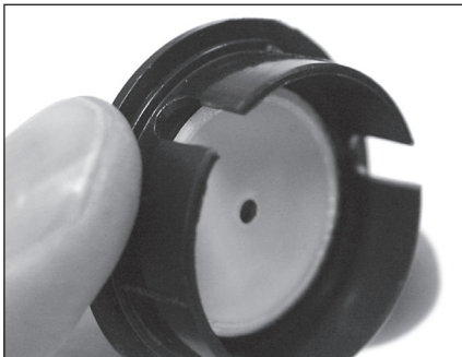
Figure 12. The quick collimation cap, which features a reflective inner surface, helps in centering reflections of the optics in the focuser during the collimation process.
