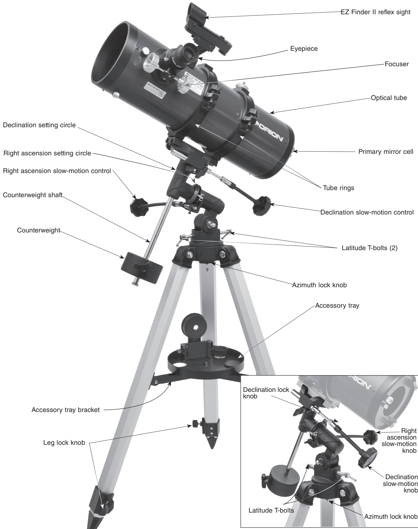
Figure 1a. The StarBlast II 4.5 EQ
